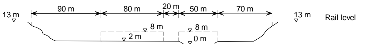
Figure 2 Elevation on the bridge centreline
