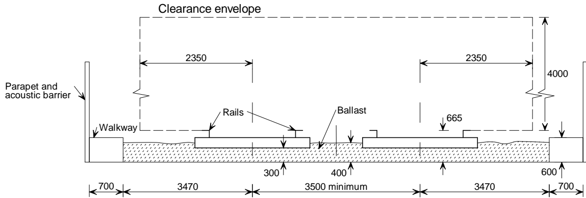
Figure 3 Cross-section of proposed bridge
